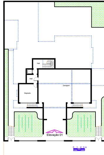
Subsolo A = 141,06 m 2
